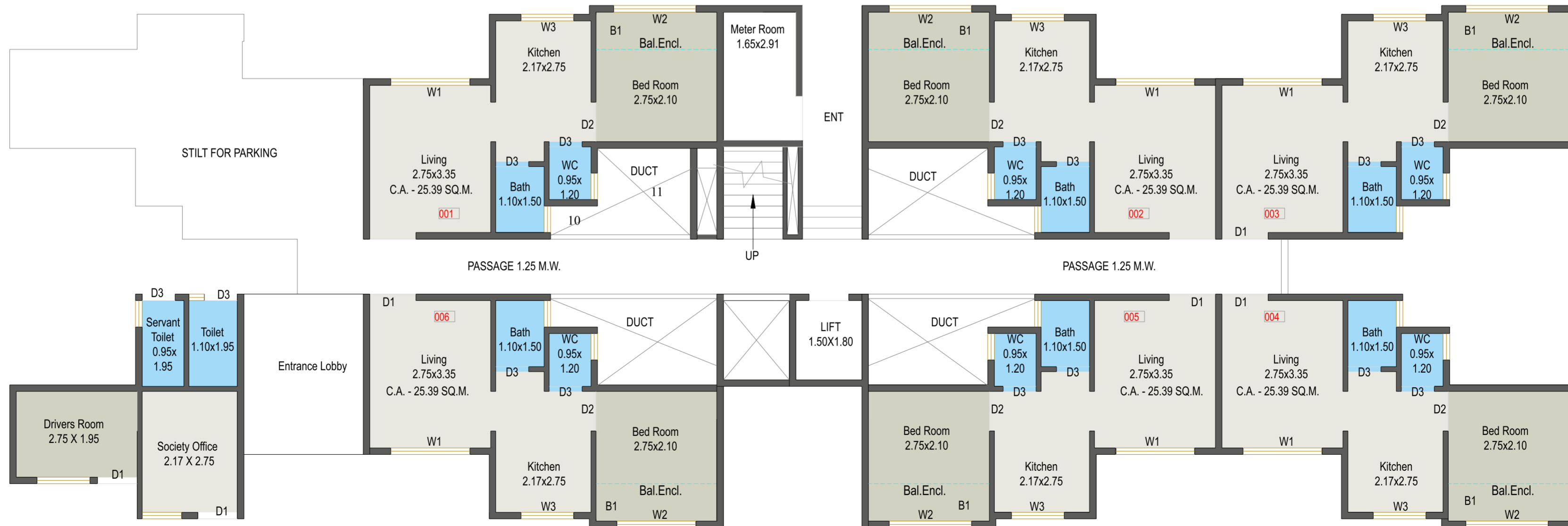
BLDG. TYP. - A GROUND FLOOR PLAN
