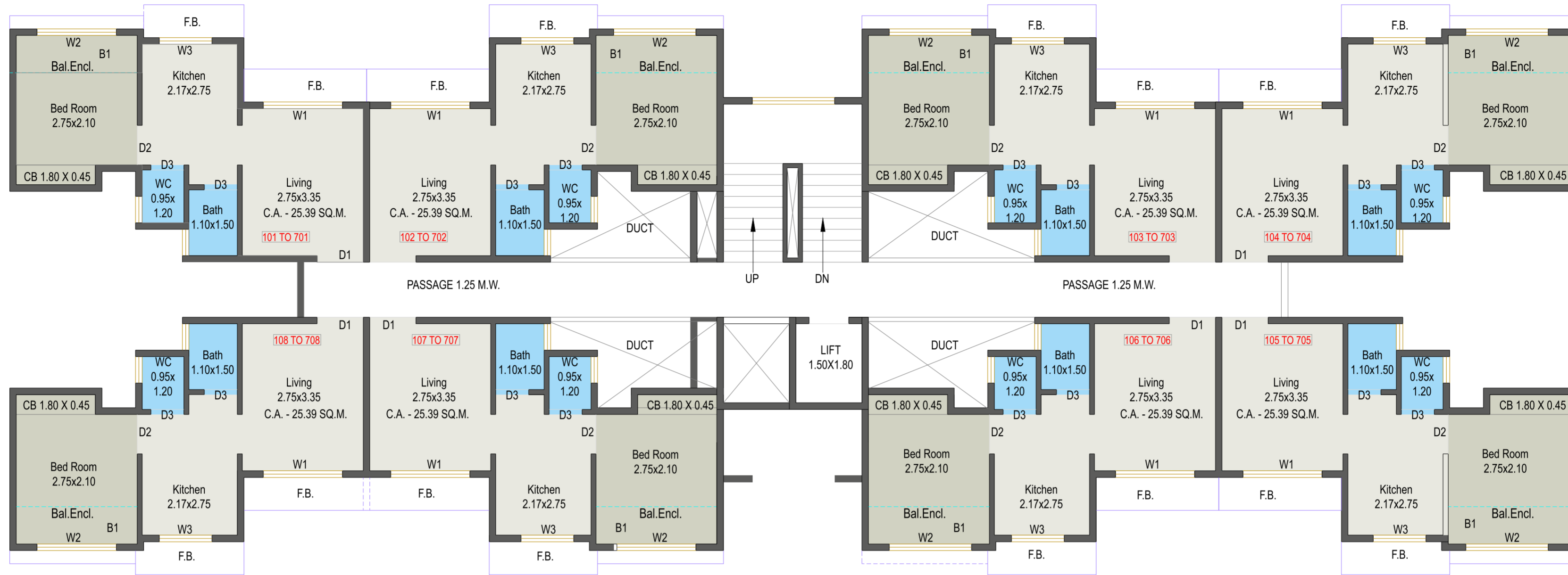
BLDG. TYP. - A 1ST TO 7TH FLOOR PLAN
